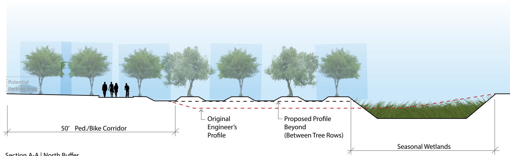
Section A-A | North Buffer
